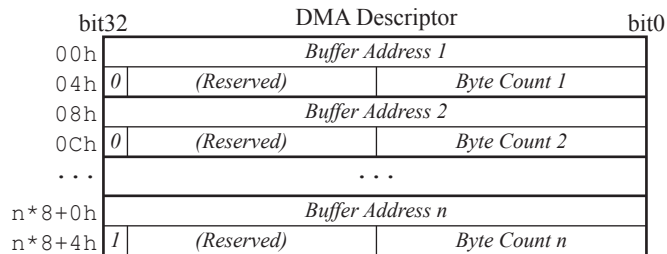
Figure 5. The structure of the DMA descriptor in ATA devices
